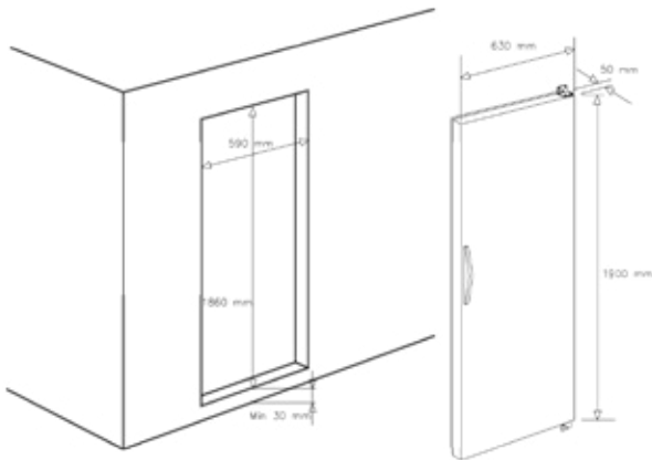
D-1900 for self build cold room or prefabricated cold room
